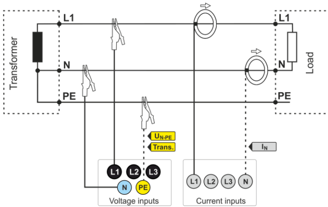
Fig. 16. Wiring diagram – single phase.
